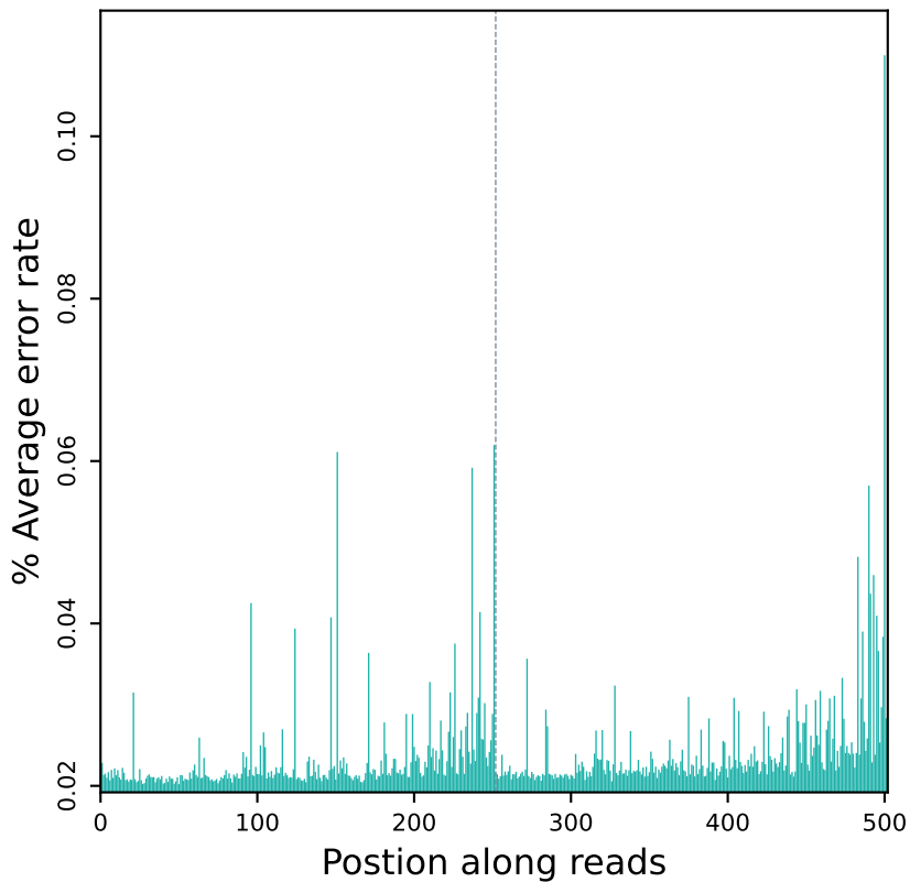
Error rate distribution along reads (R10321)
